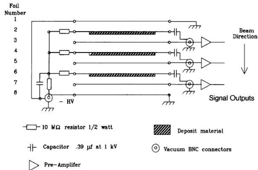
Fig. 2. Electrical wiring diagram of the ionization chamber.
