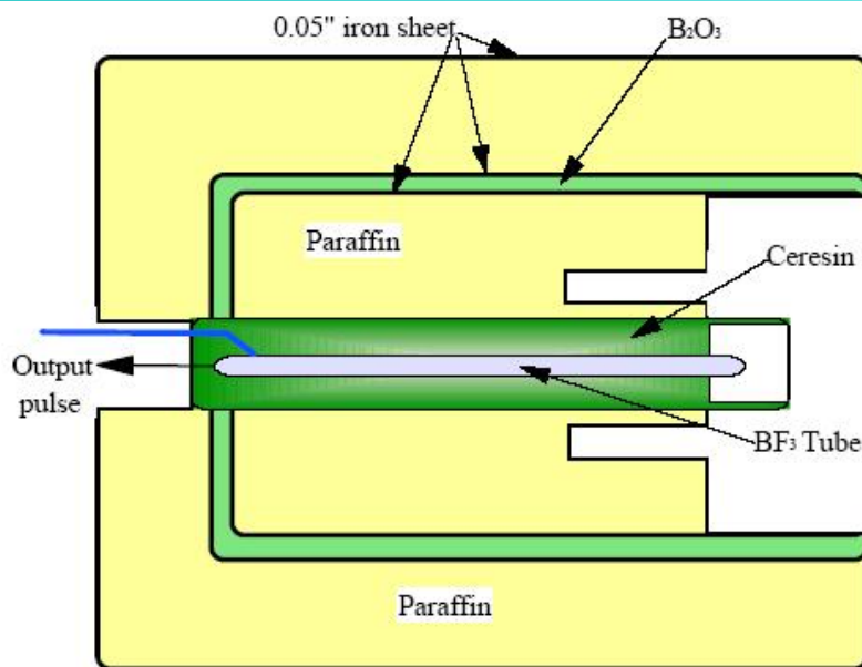
Figure 7-16. Long Counter
