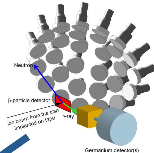
Neutron Time of Flight Spectrometer
