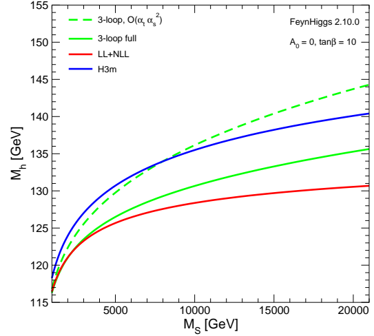
Figure 2: M_h as a function of M_S . Comparison of FeynHiggs (red) with H3m (blue). In green we show the FeynHiggs 3-loop result at O(\alpha_t\alpha_s^2) ( O(\alpha_t\alpha_s^2, \alpha_t^2\alpha_s, \alpha_t^3) ) as dashed (solid) line.
