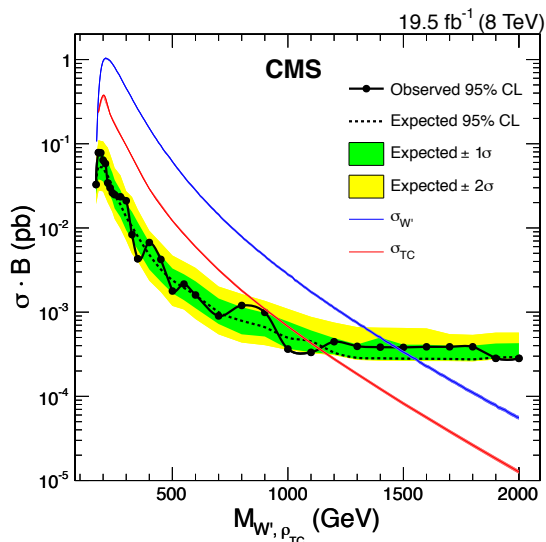
Figure 5: CMS expected and observed exclusion limit on \sigma \times \text{BR}(W \rightarrow 3\ell\nu) as a function of the WZ mass for Sequential SM W' [3] and \rho_{\text{Technicolor}} [11, 12, 13], along with the combined 1\sigma ( 2\sigma ) statistical and systematic uncertainties depicted with the green (yellow) band.
