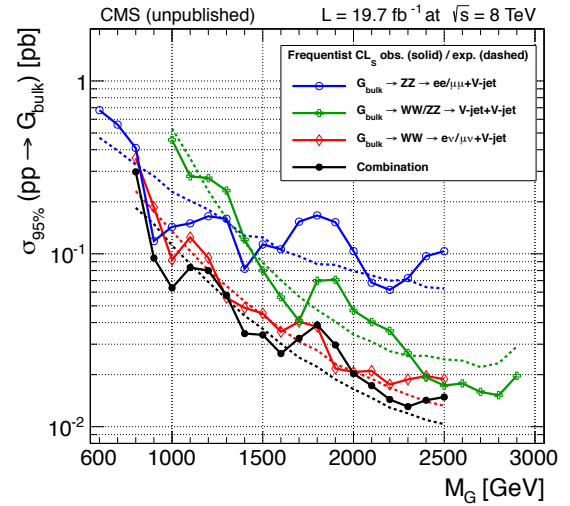
Figure 7: CMS observed (solid lines) and expected (dashed lines) 95% CL upper limit on the bulk graviton production cross section for the semi-leptonic [33], the all-hadronic channel [28], and their statistical combination. The combination is shown only in the mass range where at least two analyses contribute.
