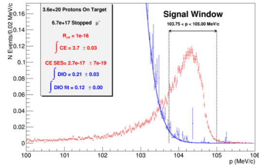
Figure 5. Momentum resolution for conversion electrons and DIO background, with a signal-to-noise ratio corresponding to R_{\mu e} of 10^{-16} .
