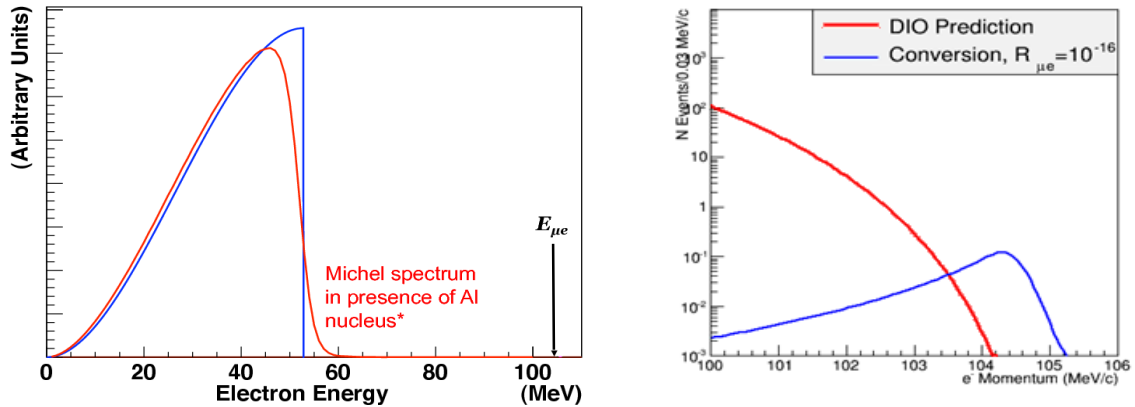
Figure 2. Left. The electron spectrum from free muon decay (blue), the spectrum of muons decaying from orbit in a muonic aluminum atom (red) and the nearly mono-energetic spectrum of conversion electrons (black). Right. The signal region. The conversion electron spectrum for a rate of 10^{-16} is shown in blue, the tail of the DIO spectrum in red.
