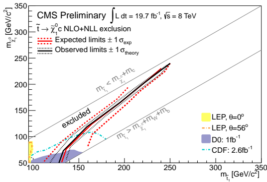
Figure 3: Observed and expected \pm 1\sigma limits on top squark production cross section in the m_{\tilde{t}_1}, m_{\tilde{\chi}_1^0} mass plane [20].
