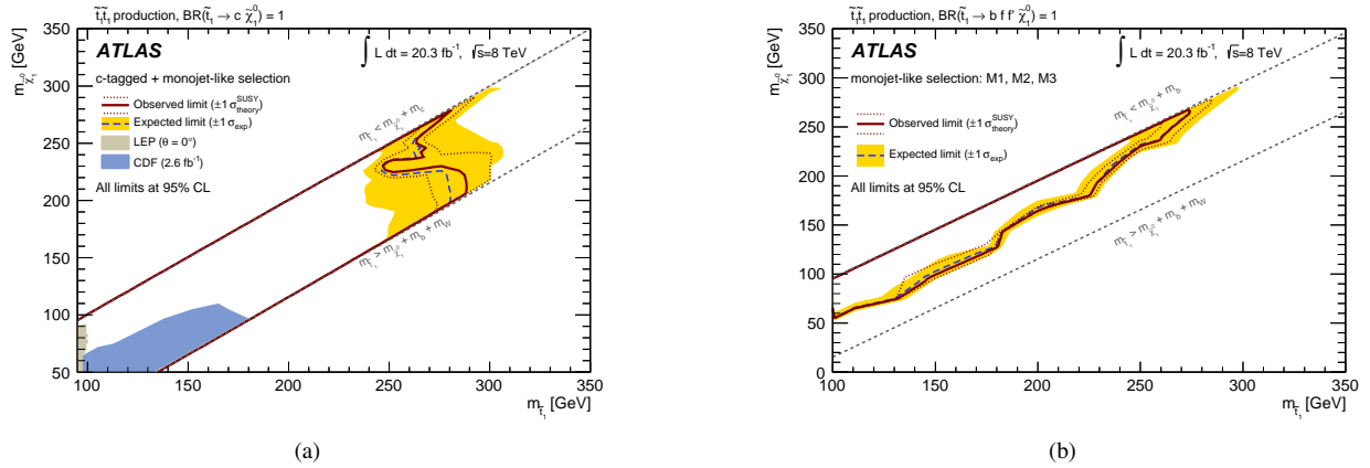
Figure 5: (a) Observed and expected \pm 1\sigma limits at 95% CL on top squark production cross section in the \tilde{t}_1, \tilde{\chi}_1^0 mass plane obtained from monojet-like and c -tagged signal regions for the case of the loop-induced decay to a charm quark. (b) Limits on the four-body decay channel obtained from the monojet-like signal regions [19].
