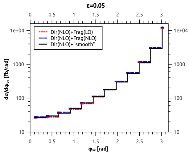
Figure 4: Angular separation between the photons \Delta\phi_{\gamma\gamma} (Right). A comparison between the different isolation criteria is shown. The applied cuts are the same as in Figs. 1, 2, and are described in the text.
