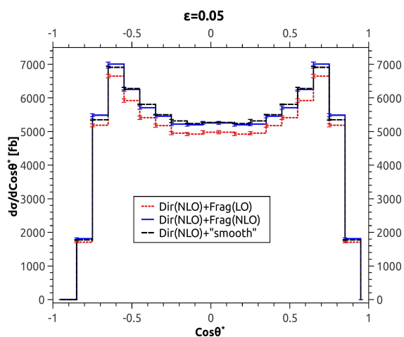
Figure 3: Diphoton cross section as a function of the \cos\theta^* . A comparison between the different isolation criteria is shown. The applied cuts are the same as in Figs. 1, 2, and are described in the text.
