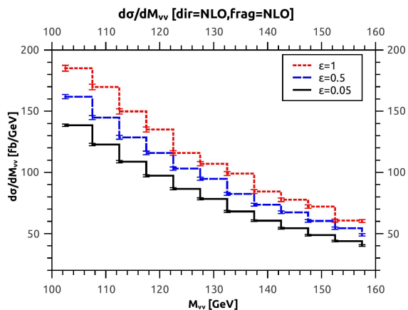
Figure 1: Diphoton cross section as a function of the invariant mass M_{\gamma\gamma} with NLO fragmentation component.
