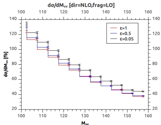
Figure 2: Diphoton cross section as a function of the invariant mass M_{\gamma\gamma} with LO fragmentation component.
