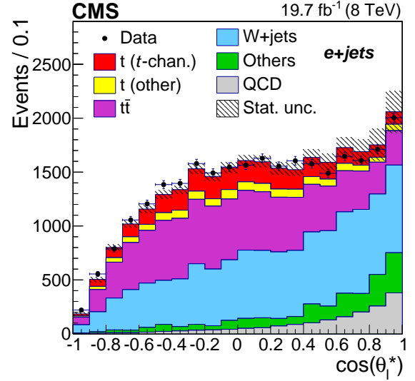
Figure 12: The reconstructed \cos\theta_l^* for data and simulation at \sqrt{s} = 8 TeV in the electron channel. The angle \theta_l^* is defined between the momentum of the down-type fermion in the W rest-frame and the W momentum in the top quark rest frame.
