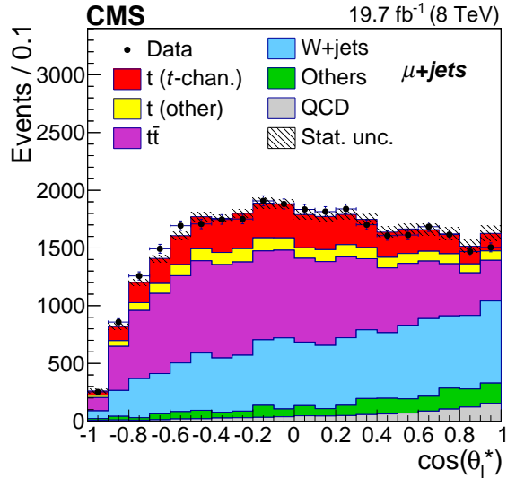
Figure 11: The reconstructed \cos\theta_l^* for data and simulation at \sqrt{s} = 8 TeV in the muon channel. The angle \theta_l^* is defined between the momentum of the down-type fermion in the W rest-frame and the W momentum in the top quark rest frame.
