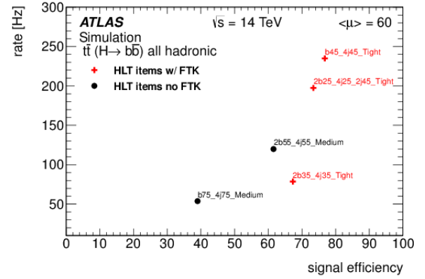
Figure 4: HLT trigger rate v.s. signal efficiency at the number of pile-up corresponds to 60 and center of mass energy 14 TeV [5]. The black points show b -jet items that will fit into the HLT constraints without FTK, red points show options with significantly larger input rates possible with FTK. All operating points assume the re-fitted FTK performance. The efficiencies are quoted with respect to the inclusive signal and include the L1 efficiency. The trigger names specify the jet multiplicities, p_T thresholds and b -tagging operating points. For example, the “2b55_4j55_Medium” trigger requires at least two medium b -tagged jets above 55 GeV and four or more jets above 55 GeV.
