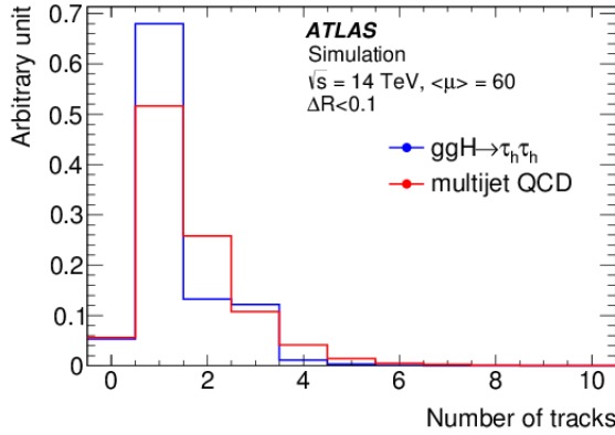
Figure 1: Number of FTK tracks inside a cone of \Delta R < 0.1 around \tau candidates [5]. A signal sample of H \rightarrow \tau_{had}\tau_{had} events is shown in blue, and a multijet QCD background sample is shown in red.
