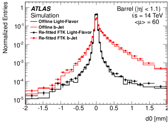
Figure 3: The transverse impact parameter distribution is shown for tracks associated to light-flavor (black) and heavy-flavor (red) jets. The solid lines show the distribution for the offline tracks, whereas the points show the FTK tracks re-fitted at HLT [5].
