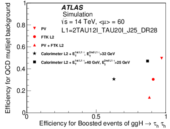
Figure 2: Efficiency of di-tau triggers for QCD multi-jet background and signal ( H \rightarrow \tau_{had}\tau_{had} ) under the number of pile-ups corresponds to 60 and center-of-mass energy 14 TeV [5]. The red downwards pointing triangle shows the per event efficiency of the HLT selection which requires that the jet and at least one of the two \tau s to be consistent with the primary vertex (PV). The red circle shows the per event efficiency for applying the FTK selection at HLT. The red upwards pointing triangle show the per event efficiency for applying the FTK selection at HLT and the primary vertex consistency requirement. The black star shows the efficiency of applying the calorimeter cluster selection and adding the requirement that both the Level-1 tau candidates have E_T > 32 GeV. The black triangle shows the efficiency for the same selection described above but with Level-1 \tau candidates satisfying E_T > 40 GeV for the first and E_T > 25 GeV for the second.
